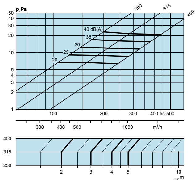
EAGLE D 250, 315, 400
