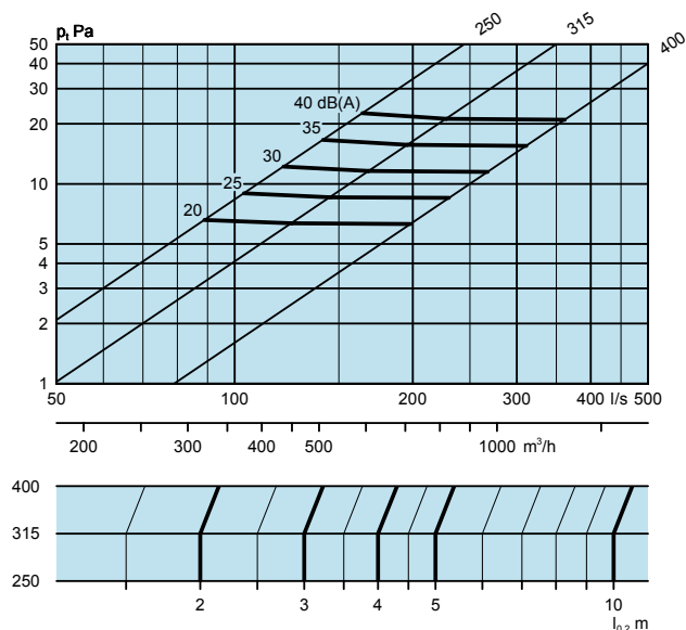
EAGLE D 250, 315, 400
