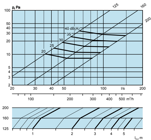
EAGLE D 125, 160, 200
