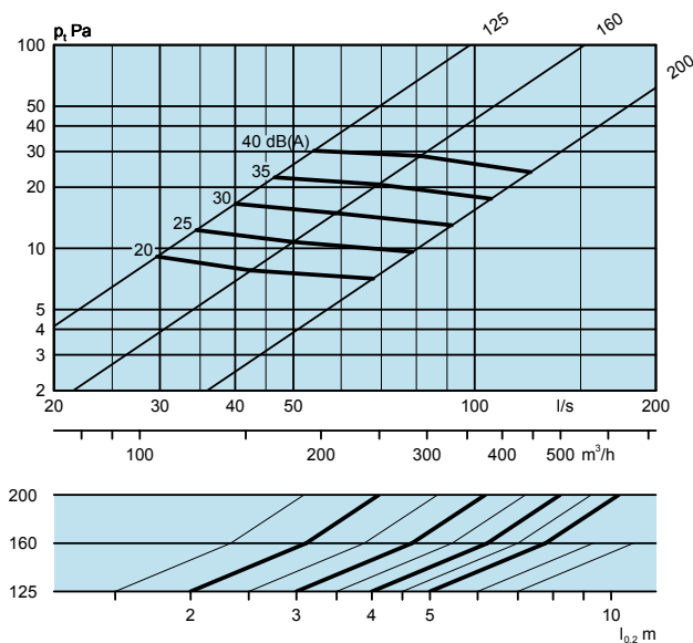
EAGLE S 125, 160, 200
